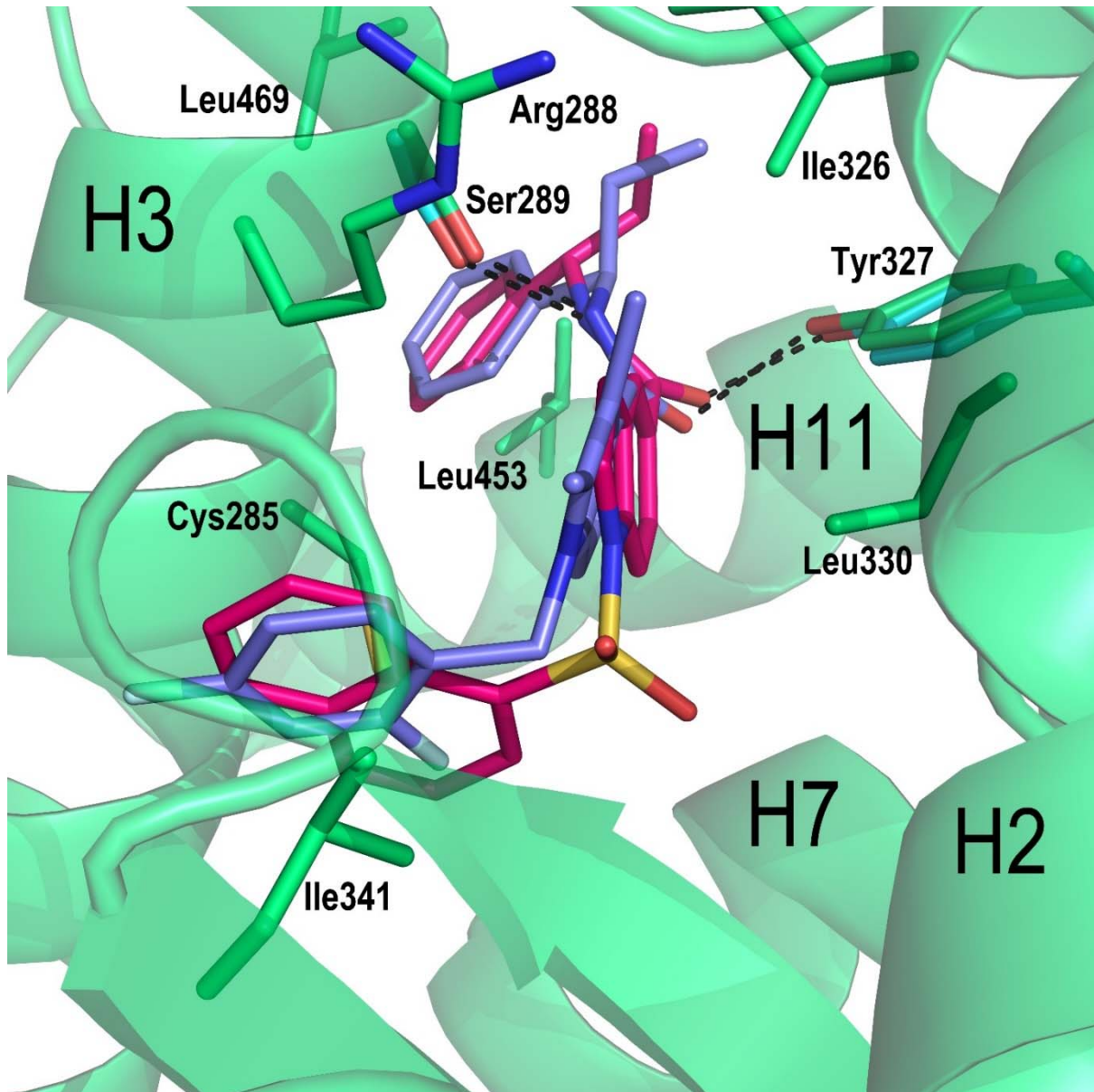
Supplementary Figure 2: Comparison of ligand binding modes of SR1988 and SR2067 as determined by their crystal structures. The PPAR \gamma LBD main chain is represented in green ribbons, with side chains of interacting residues shown in green sticks. SR1988 is shown in purple sticks, and SR2067 is represented as pink sticks.
